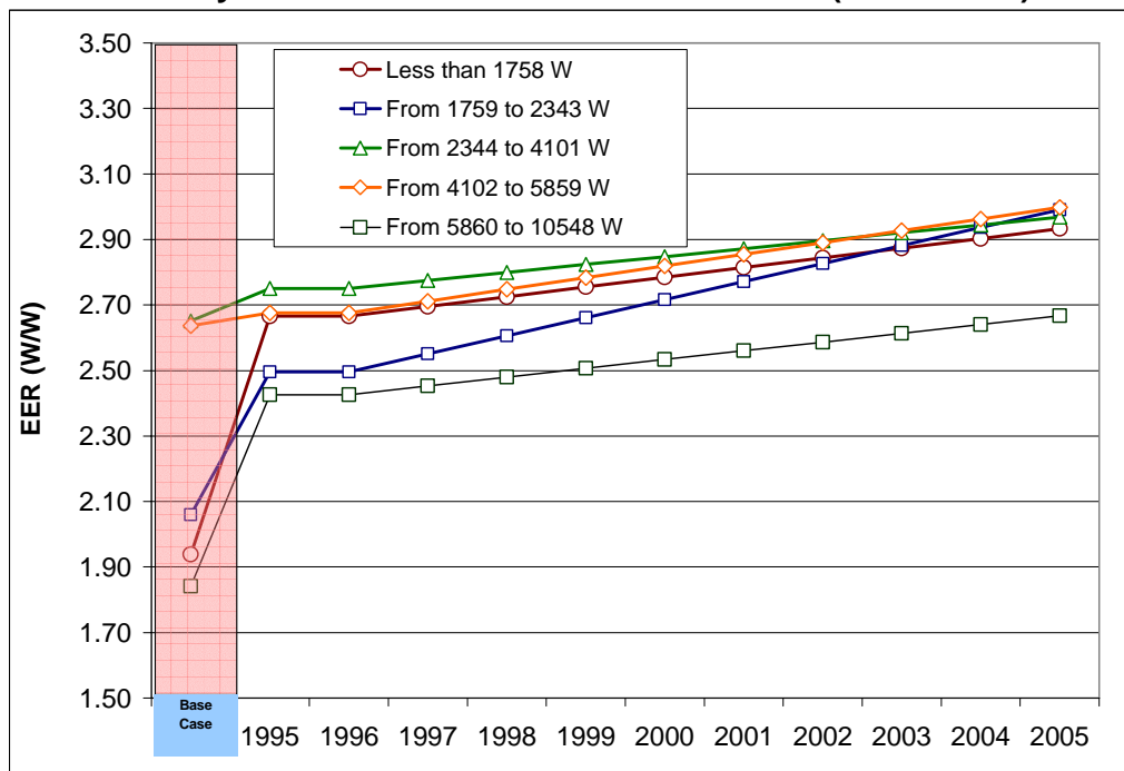
Figure 7 – Efficiency of Air Conditioner Product Classes (Watts/Watt)
