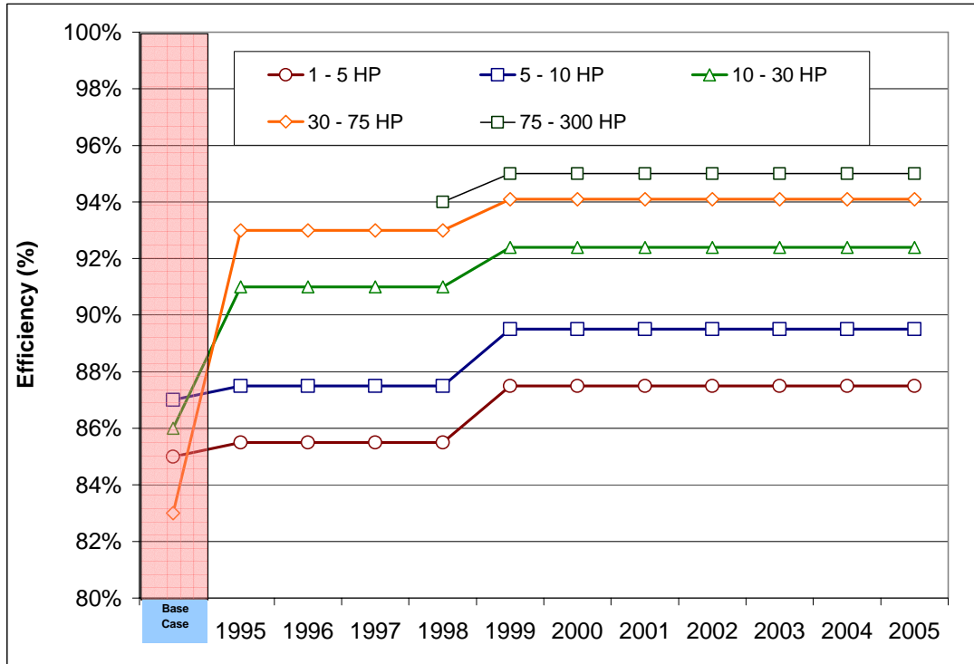
Figure 11 - Efficiency of Three Phase Motors Product Classes
