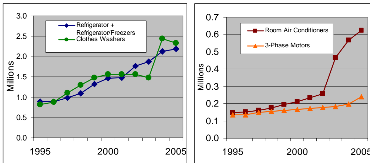
Figure 2 – Product Shipments 1995-2004
